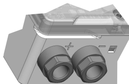
Connection nozzle with inner thread G \frac{1}{8}
